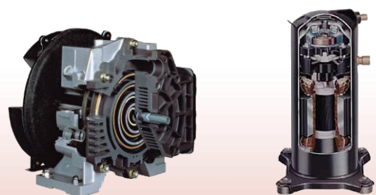
HVAC system
